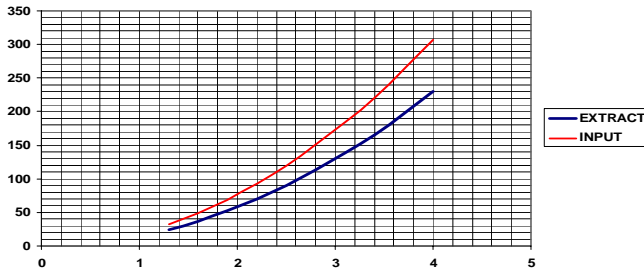
TYPICAL RESISTANCE WHEN USED AS TERMINAL ONLY SIZE 500/560
